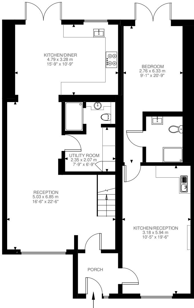
Ground Floor 1035 ft 2
